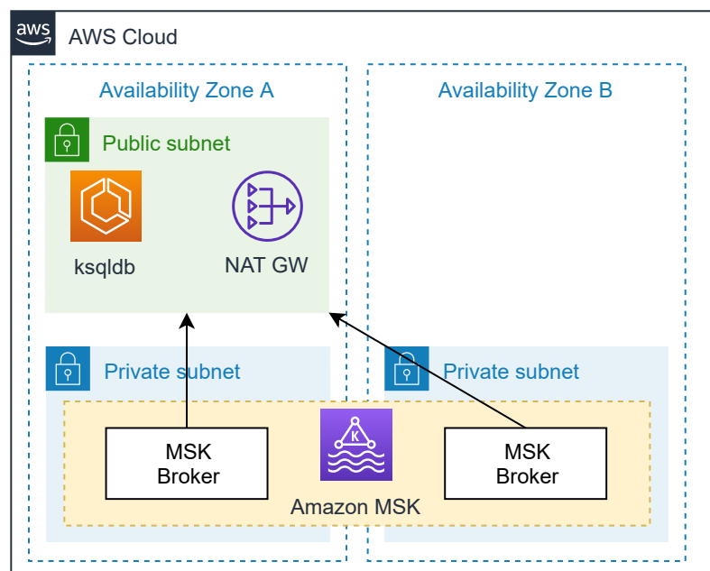
Abb. 26: Networking MSK
